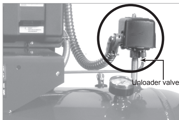
Figure 9 - Pressure Switch
